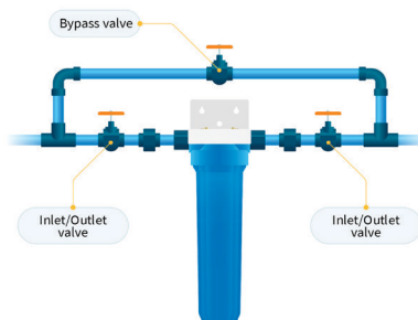
Recommended Installation Diagram
